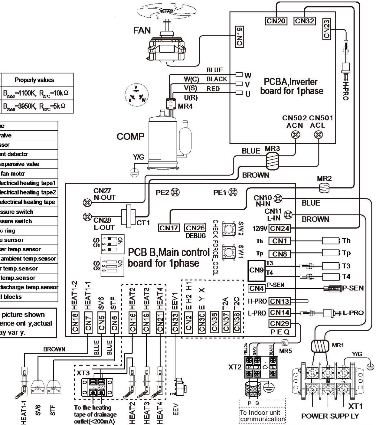
Figure 2-4.1: NXHPS-V12(14,16)W/D2N8-B wiring diagram
