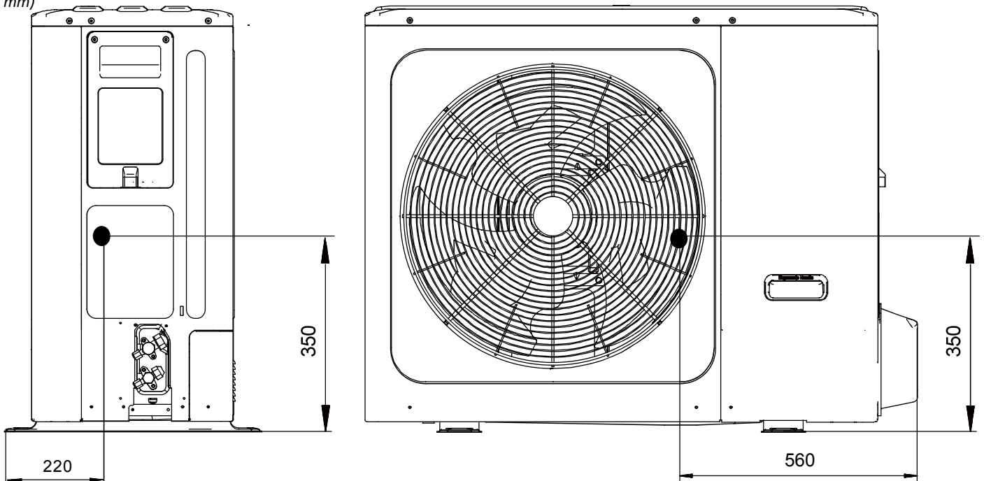
Figure 2-2.2: NXHPS-V8(10)W/D2N8-B dimensions and center of gravity (unit: mm)
