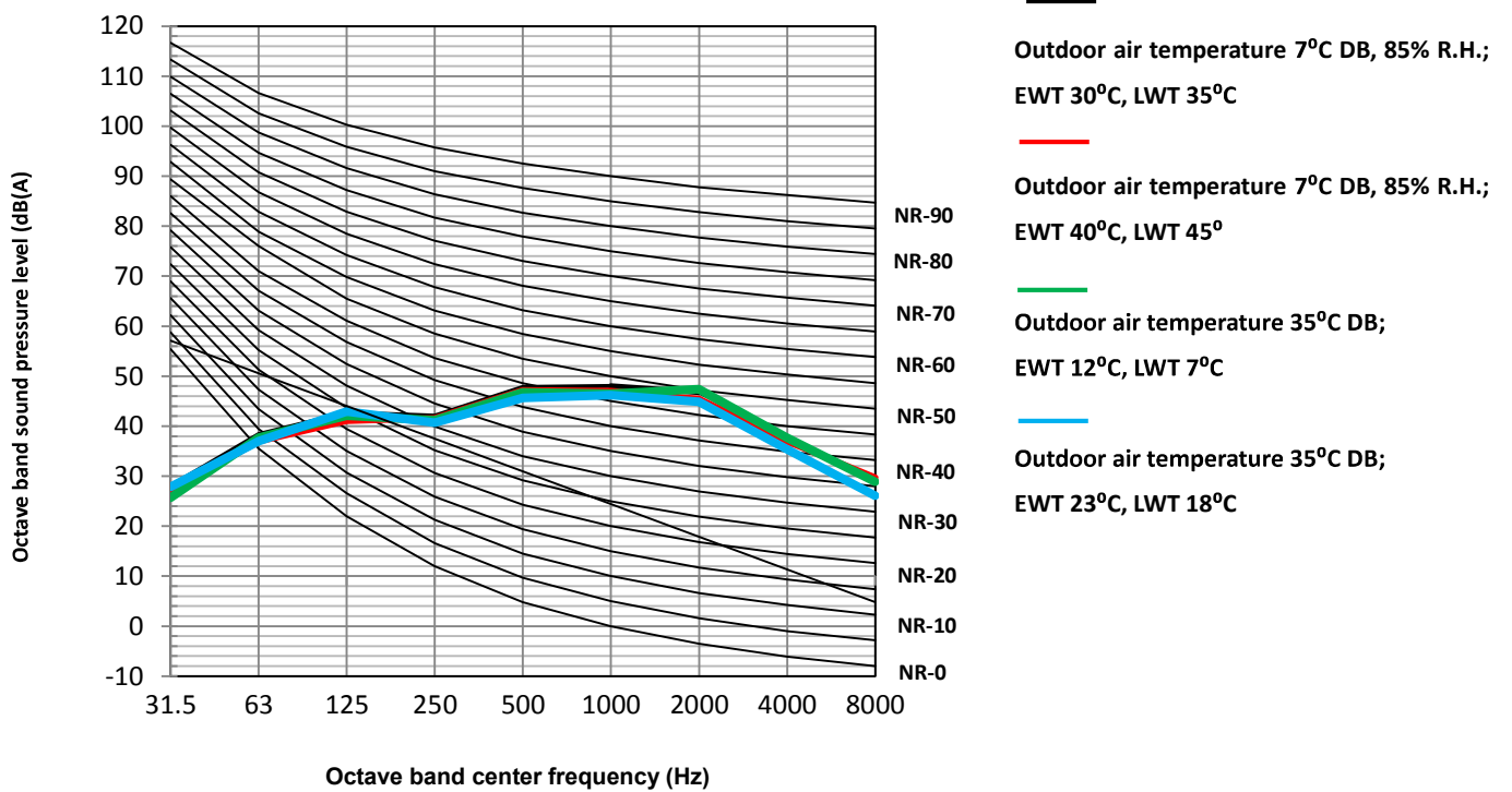
Figure 2-8.5: NXHPS-V14/D2N8-B octave band levels
