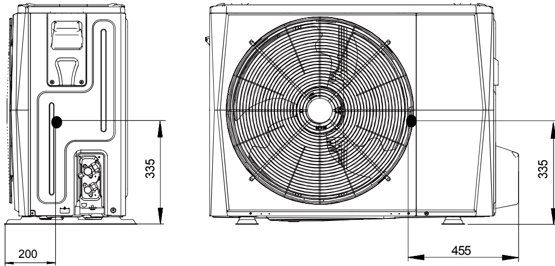
Figure 2-2.1: NXHPS-V4(6)W/D2N8-B dimensions and center of gravity (unit: mm)
