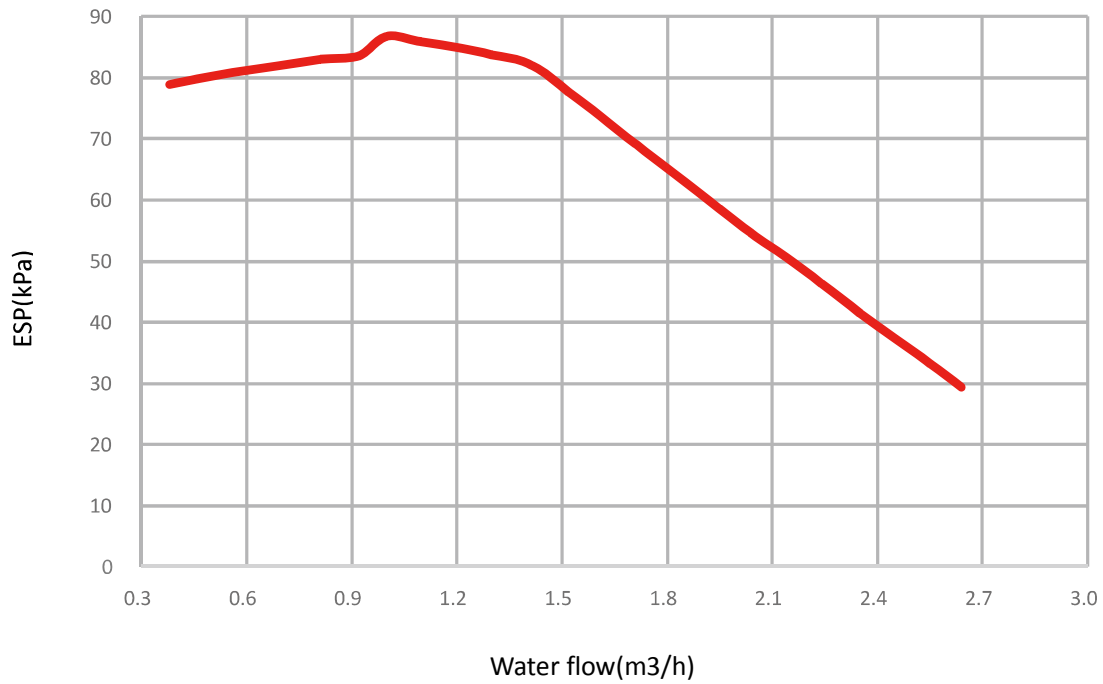
Figure 2-7.1: NXHB-A60(100)/CD***GN8-B hydronic performance
