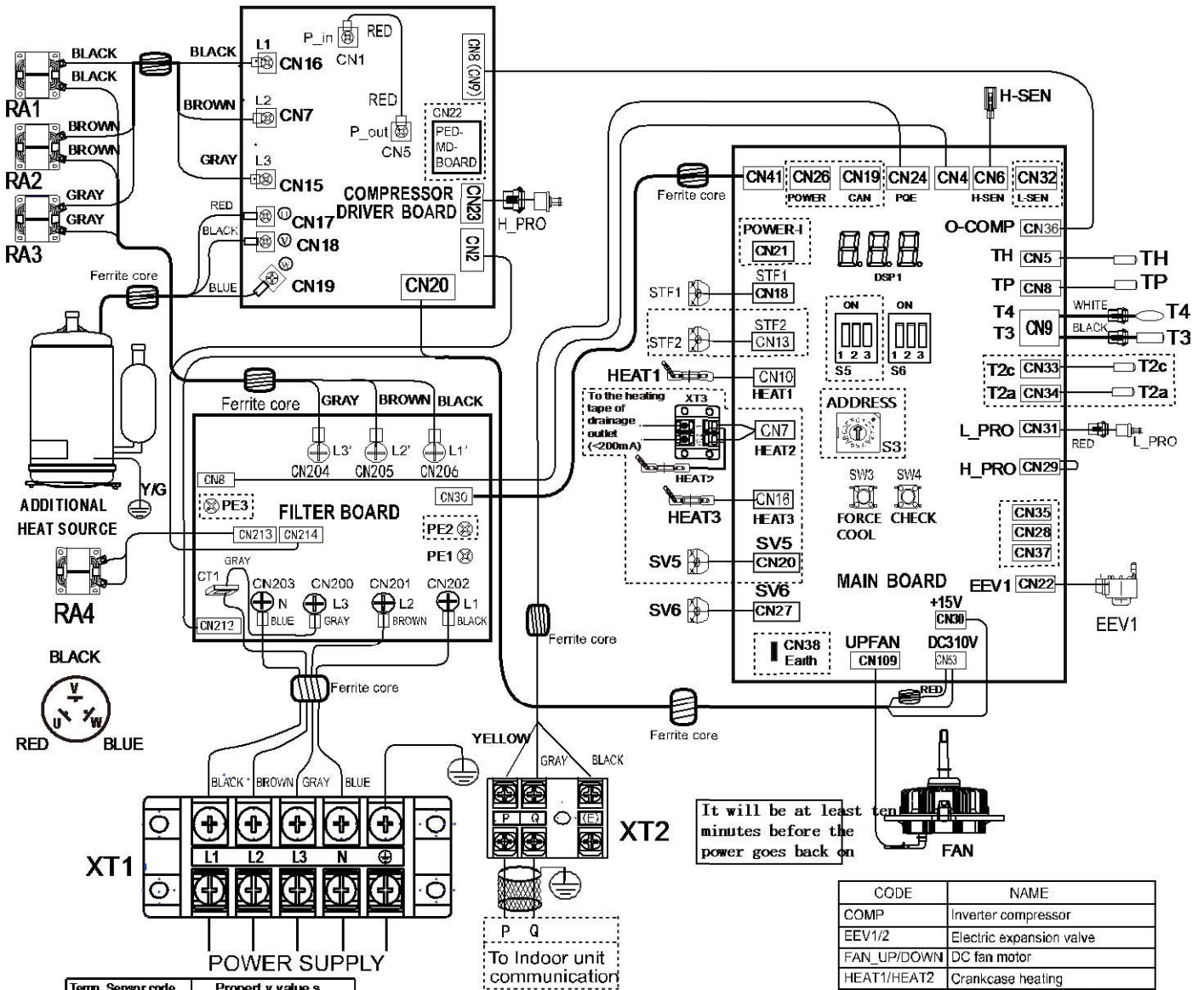
Figure 2-4.1: NXHPS-V12(14,16)W/D2RN8-B wiring diagram
