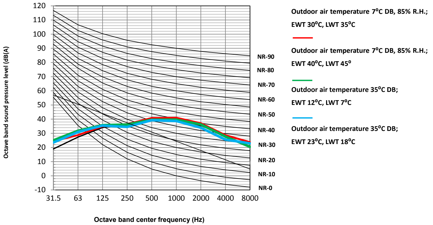
Figure 2-8.2: NXHPS-V4/D2N8-B octave band levels
