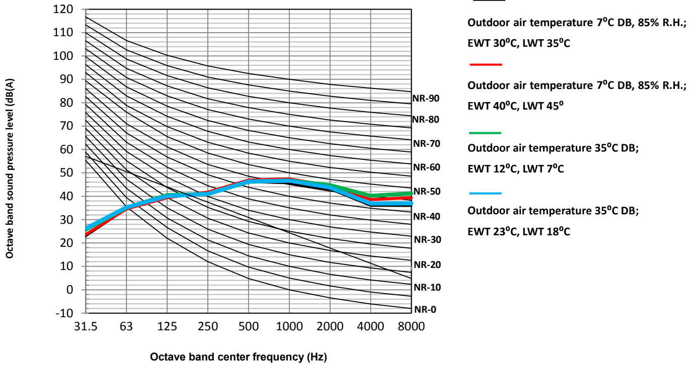
Figure 2-8.5: NXHPS-V12/D2RN8-B octave band levels
