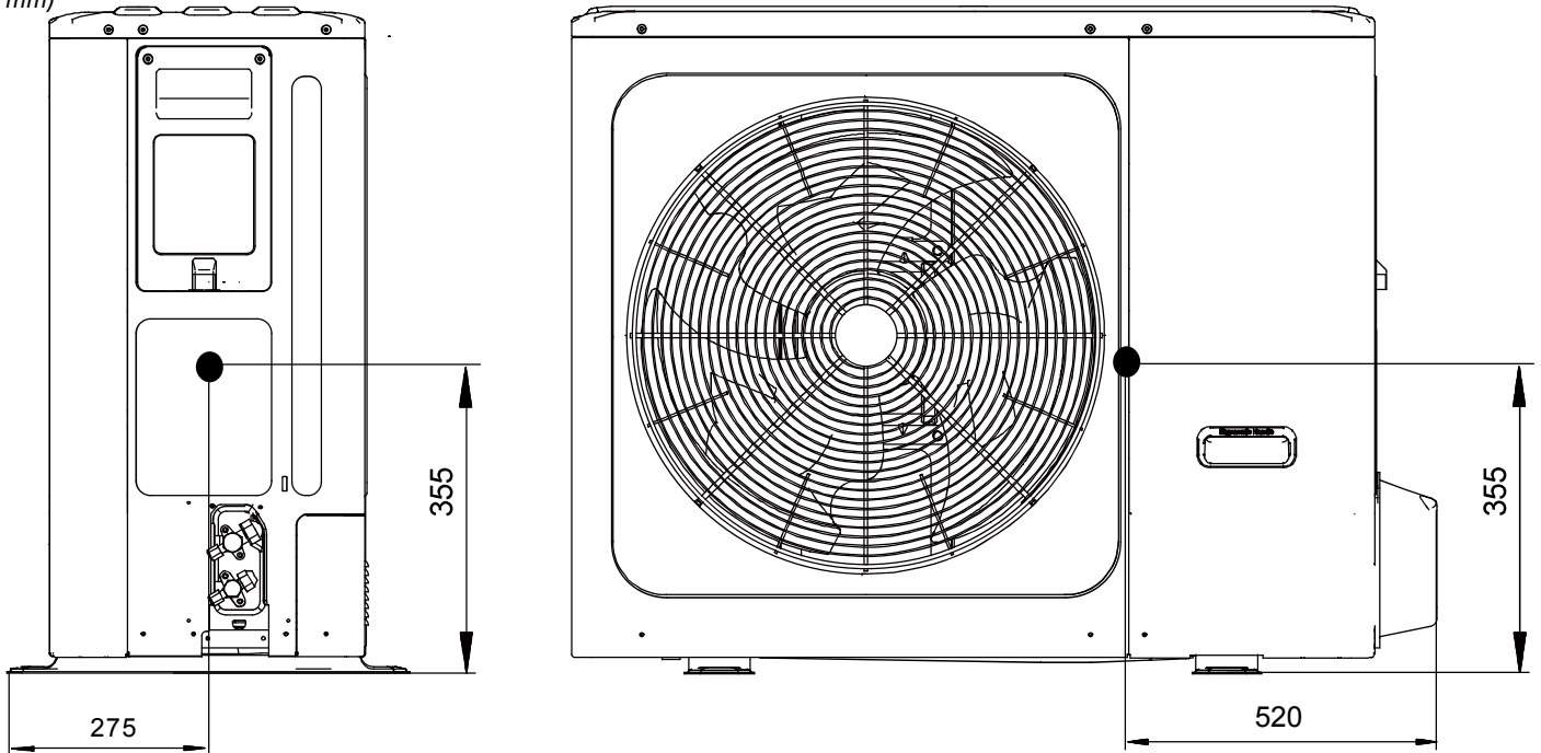
Figure 2-2.2: NXHPS-V12(14,16)W/D2N8-B dimensions and center of gravity (unit: mm)
