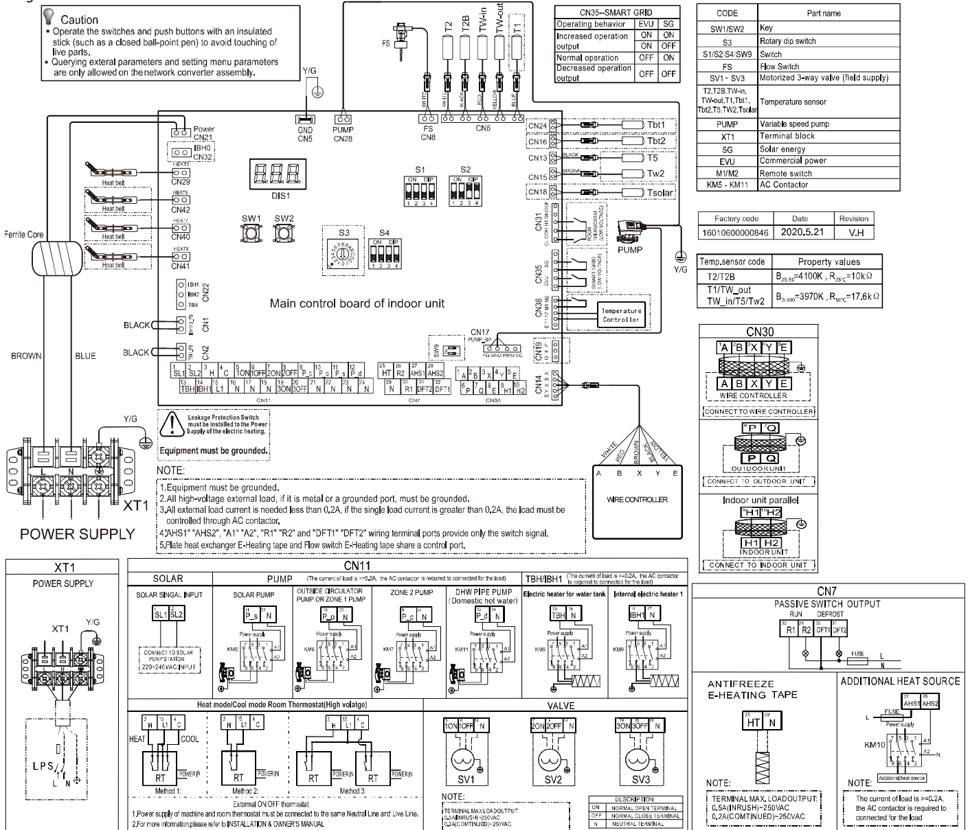
Figure 2-4.2 NXHB-A60(100,160)/CGN8-B wiring diagram
