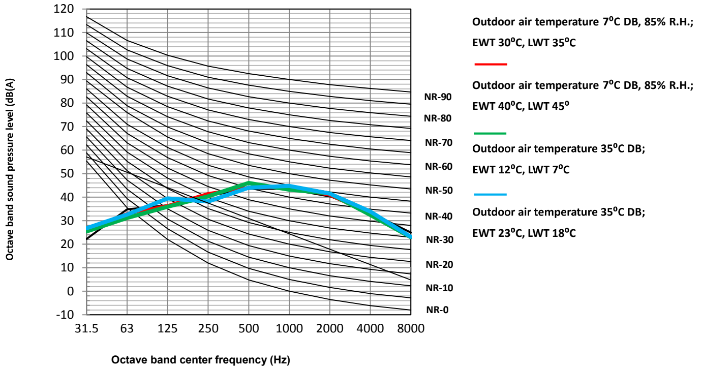
Figure 2-8.4: NXHPS-V8/D2N8-B octave band levels
