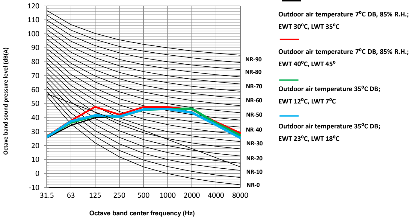
Figure 2-8.5: NXHPS-V12/D2N8-B octave band levels
