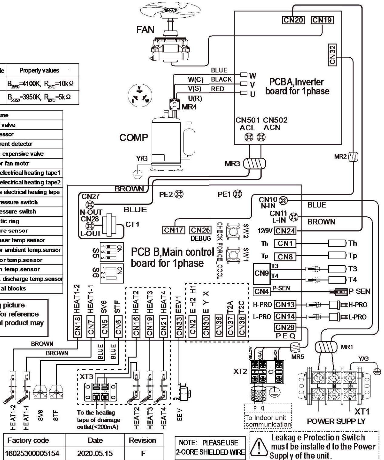
Figure 2-4.1: NXHPS-V4(6, 8, 10)W/D2N8-B wiring diagram
