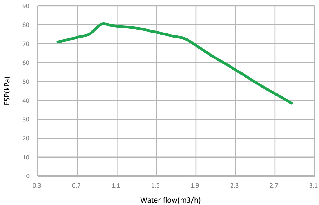
Figure 2-7.2: NXHB-A160/CDS90GN8-B hydronic performance
