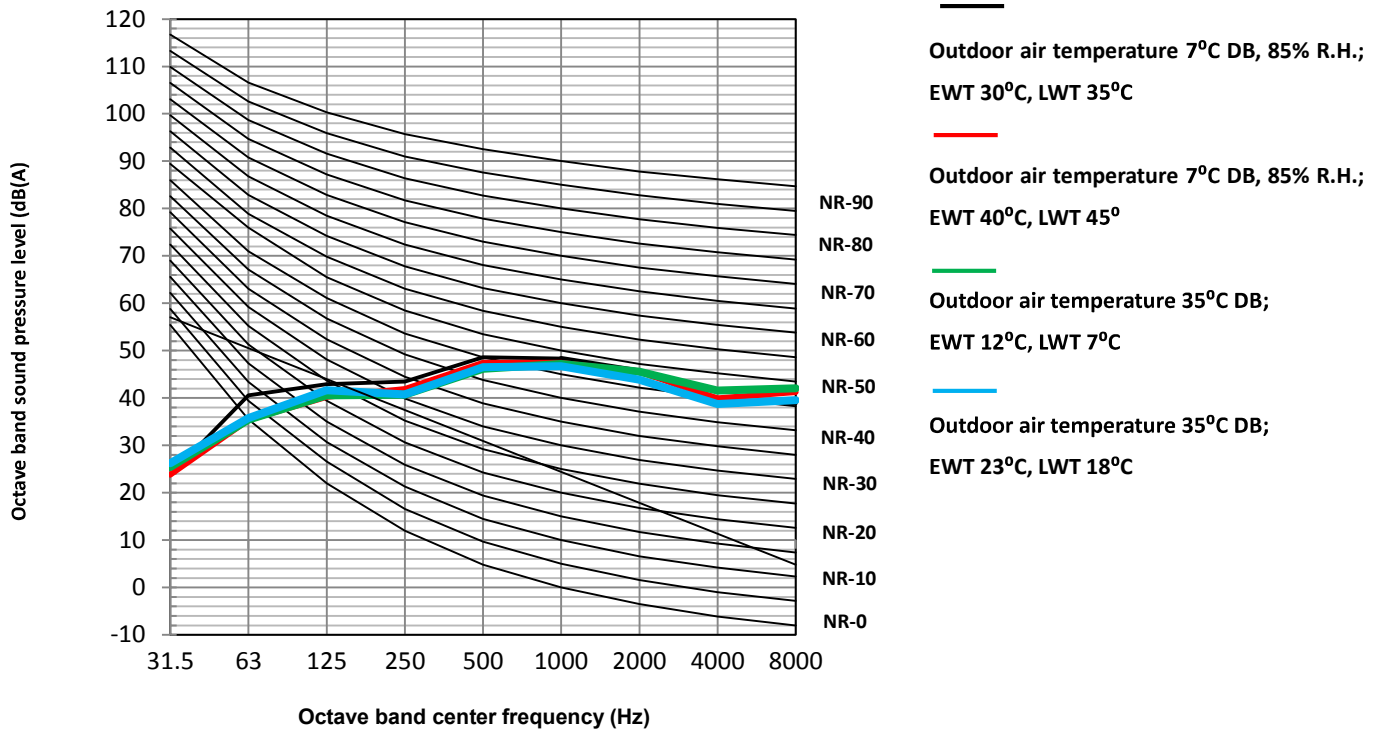
Figure 2-8.5: NXHPS-V14/D2RN8-B octave band levels
