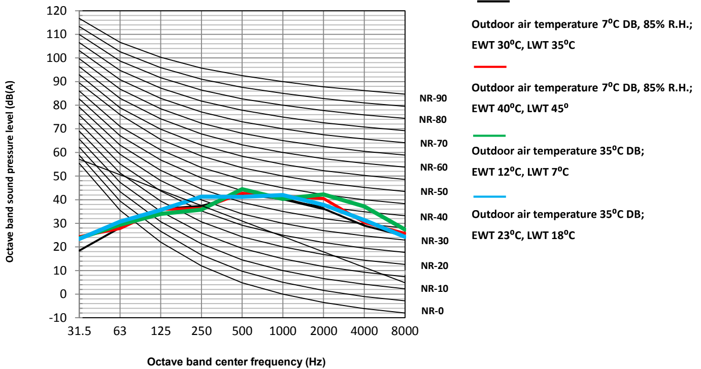
Figure 2-8.3: NXHPS-V6/D2N8-B octave band levels
