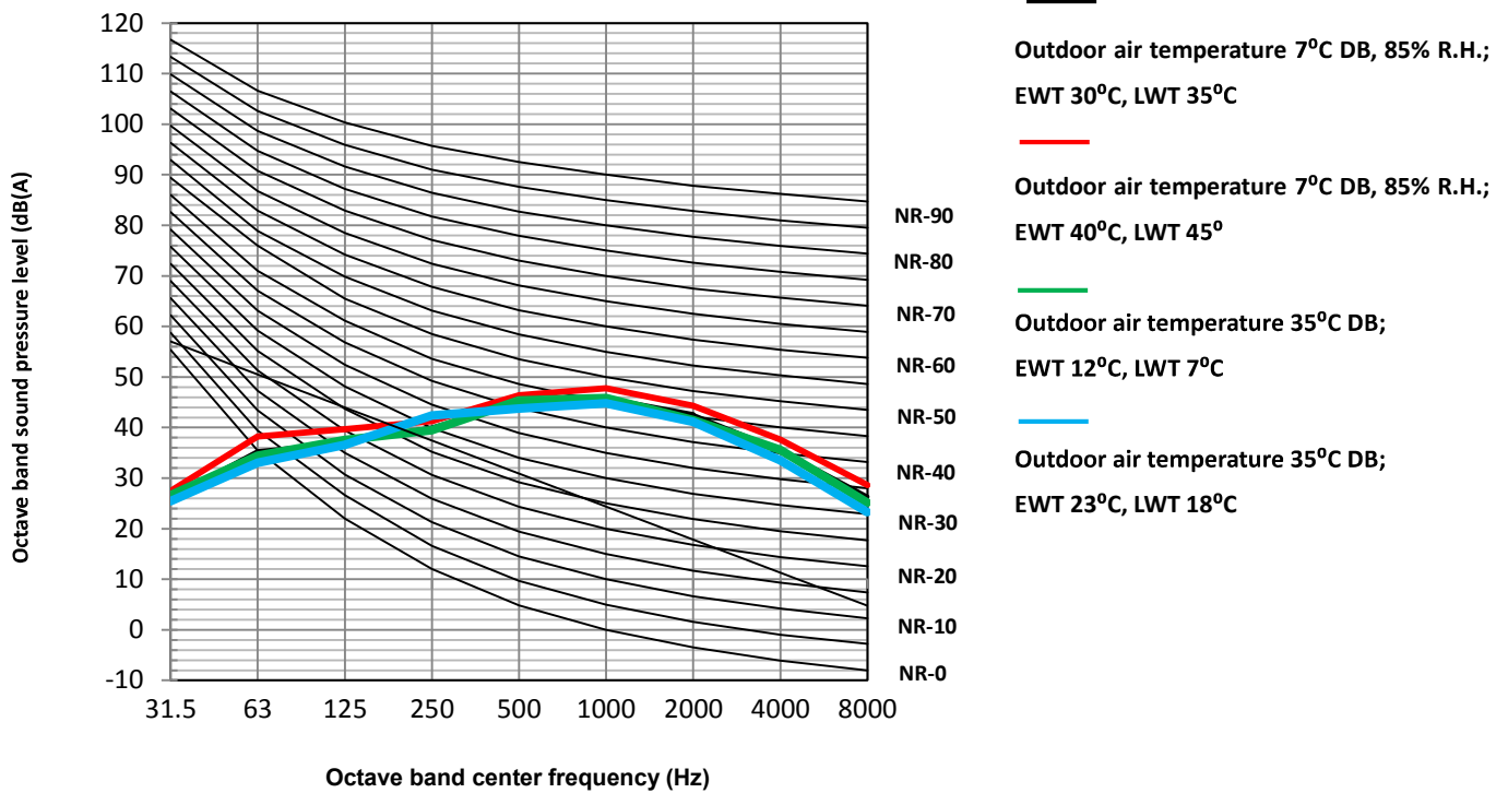
Figure 2-8.5: NXHPS-V10/D2N8-B octave band levels
