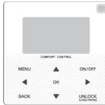
Figure 3-8.1: User interface
