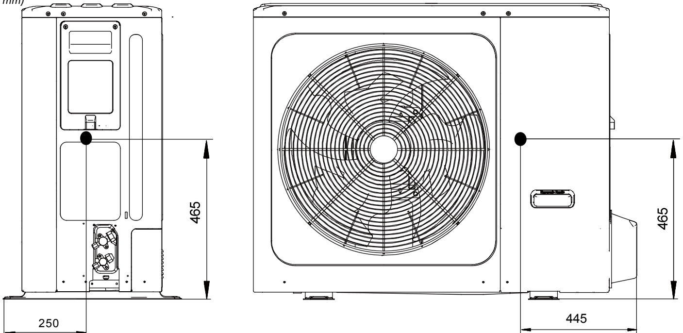
Figure 2-2.2: NXHPS-V12(14,16)W/D2RN8-B dimensions and center of gravity (unit: mm)
